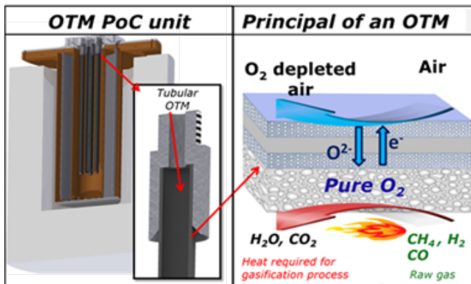
Figure 5. Operating principle of an oxygen transport membrane.
