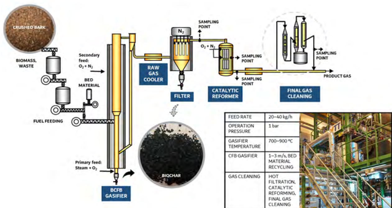
Figure 4. BCFB gasification pilot at VTT's Piloting Centre Bioruukki, Finland.
