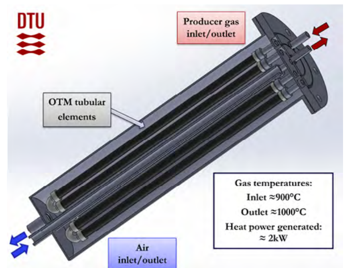
Figure 7. The core unit of the OTM reactor.
